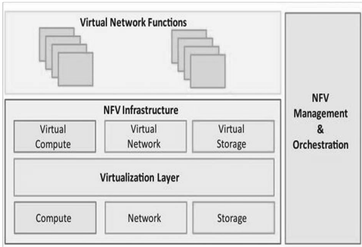
NFV Architecture
